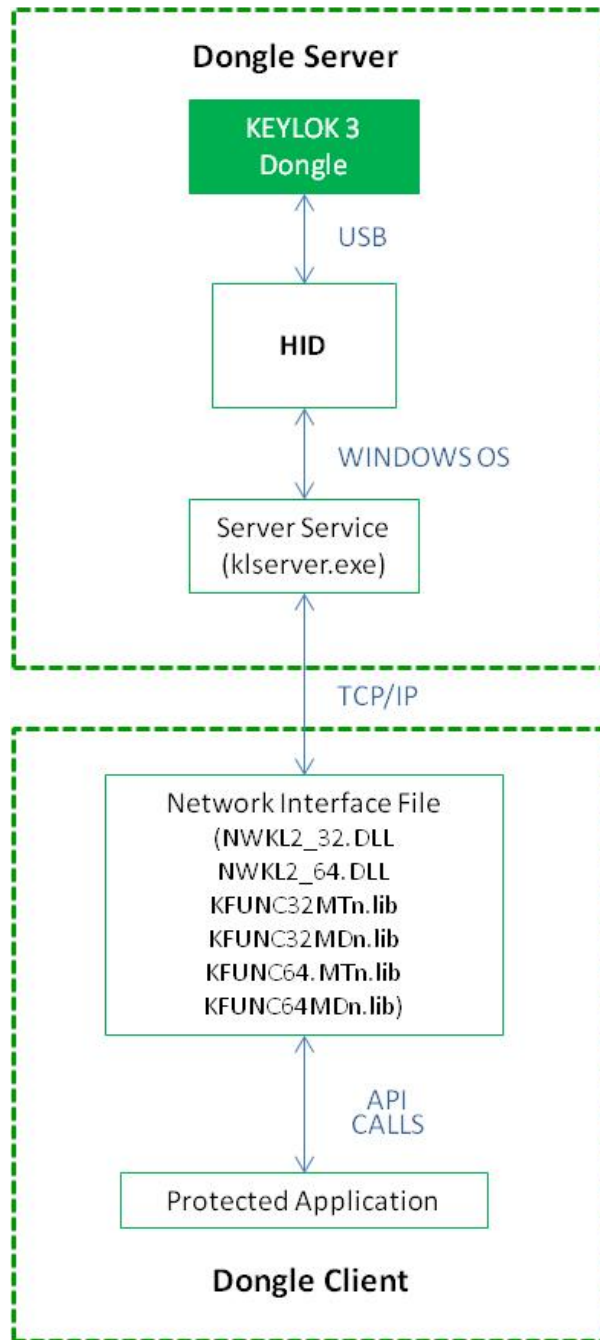
Figure 2: Dongle Access over a TCP/IP network
