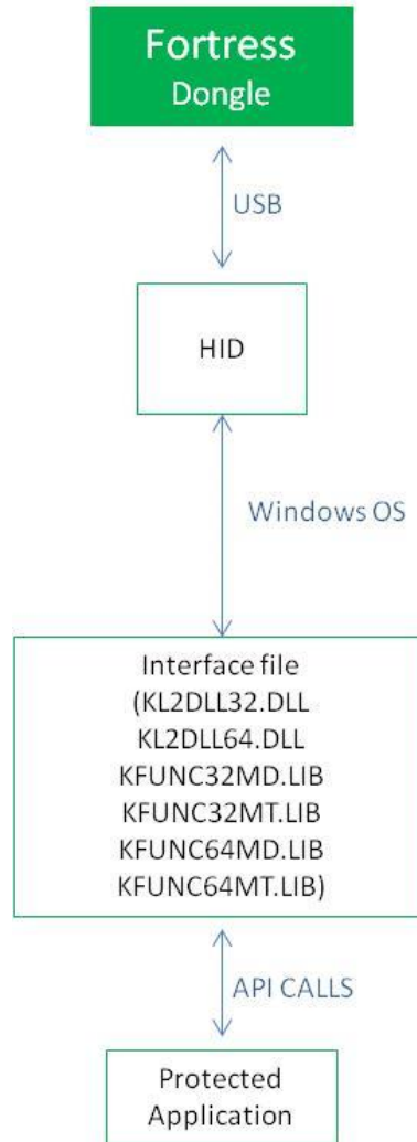
Figure 1: How Dongles Communicate with a Protected Application
